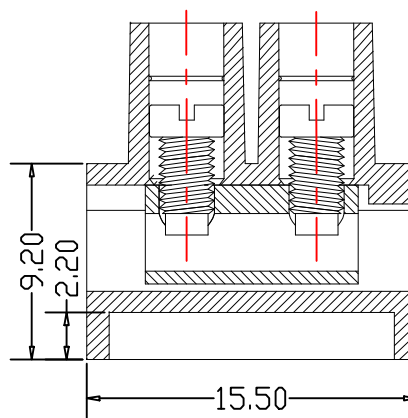
W/O Wire Cage Type1
