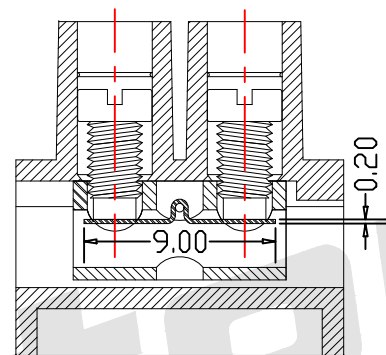
With Wire Cage Type2
